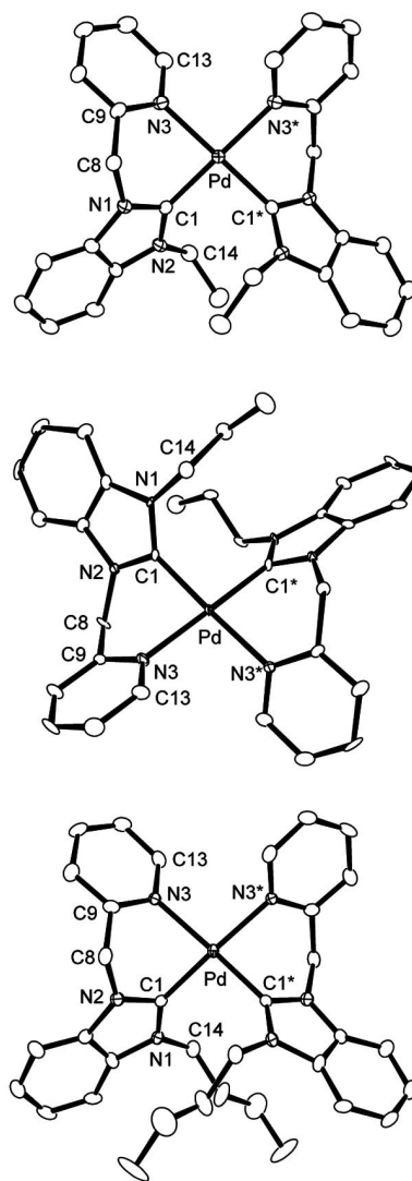
Figure 2. Molecular structures of the dicationic palladium complexes in 7 (top), 8 ·2MeOH (middle), and 9 ·2H 2 O (bottom). Hydrogen atoms, bromide counterions, and solvent molecules have been omitted for clarity.
