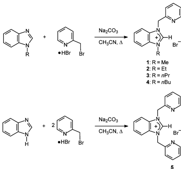
Scheme 1. Synthesis of the picoline-functionalized benzimidazolium salts 1–5 .
