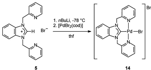
Scheme 3. Preparation of the pincer-type palladium complex 14 .
