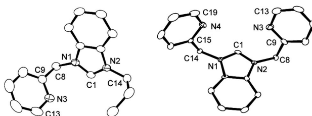
Figure 1. Molecular structures of the picoline-functionalized benzimidazolium cations in 3 and 5 ·H 2 O. Hydrogen atoms, the bromide counteranion, and solvent molecules have been omitted for clarity. Selected bond lengths [Å] and angles [°] in 3 : N1–C1 1.328(3), N1–C8 1.464(4), N2–C1 1.328(3), N2–C14 1.472(3), N3–C9 1.341(4), N3–C13 1.335(4); N1–C1–N2 110.4(2), N1–C8–C9 110.3(2), C9–N3–C13 116.7(3). Selected bond lengths [Å] and angles [°] in 5 ·H 2 O: N1–C1 1.318(6), N1–C14 1.468(6), N2–C1 1.325(7), N2–C8 1.462(6), N3–C9 1.341(7), N3–C13 1.346(7), N4–C15 1.342(6), N4–C19 1.344(7); N1–C1–C2 111.6(5), N2–C8–C9 111.2(4), N1–C14–C15 110.8(4), C9–N3–C13 116.7(5), C15–N4–C19 116.3(5).
