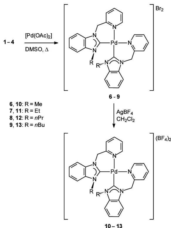
Scheme 2. Synthesis of palladium complexes with picoline-functionalized benzimidazolin-2-ylidene ligands.
