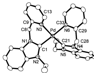
Figure 3. Molecular structure of the dicationic palladium complex in 11 ·CH 2 Cl 2 . Hydrogen atoms and the two tetrafluoroborate anions have been omitted for clarity.
